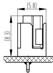
Assembly view (TJC20041-nA&TJC20041-nY) (FYI) Assembly view (TJC20041-nA&TJC20041-nY) (FYI)
