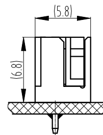
Assembly view (TJC20041-nA&TJC20041-nY) (FYI) Assembly view (TJC20041-nA&TJC20041-nY) (FYI)
