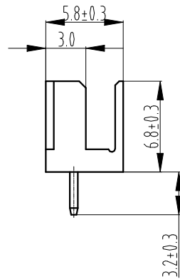
Assembly view (TJC20041-nA&TJC20041-nY) (FYI) Assembly view (TJC20041-nA&TJC20041-nY) (FYI)
