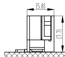
Assembly view (TJC20041-nAW&TJC20041-nYI) (FYI)
