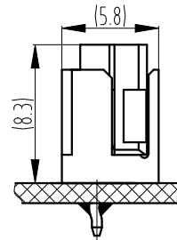
Assembly view (TJC20041-nAK&TJC20041-nYI) (FYI)
