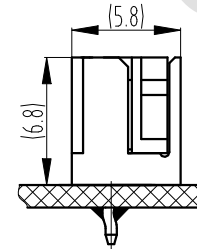
Assembly view (TJC20027-nAK&TJC20041-nYI) (FYI)
