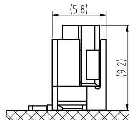
Assembly view (TJC20041-nAW&TJC20041-nY) (FYI)
