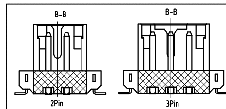
Assembly view (TJC20041-nAW&TJC20041-nYI) (FYI)
