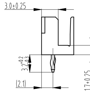
Assembly view (TJC20041-nAK&TJC20041-nYI) (FYI)
