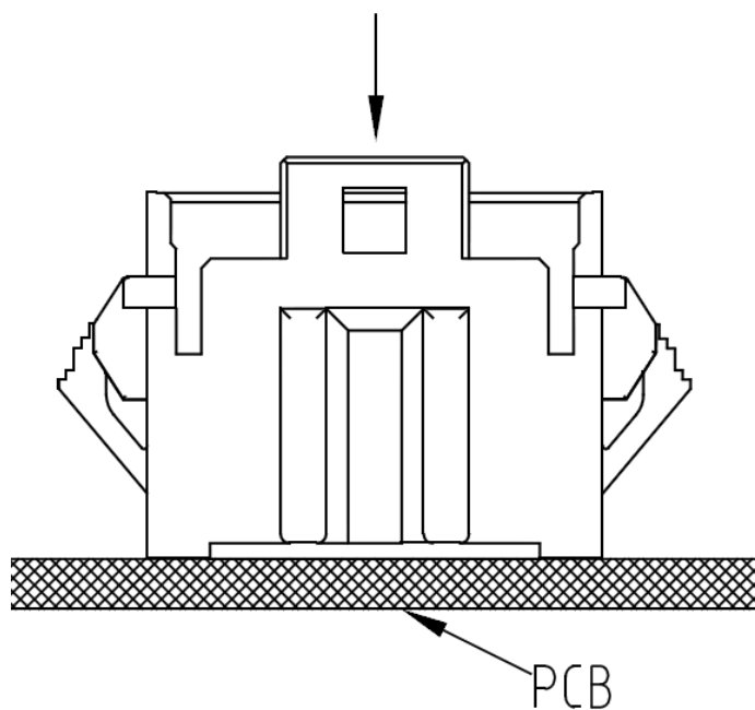
Fig.3 Panel mating force measurement direction
