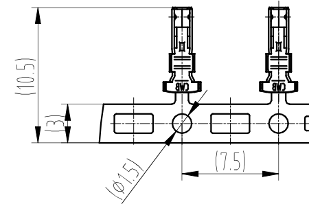
Contact view 1:2
