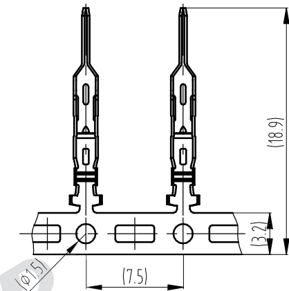
Contact view 1:2
