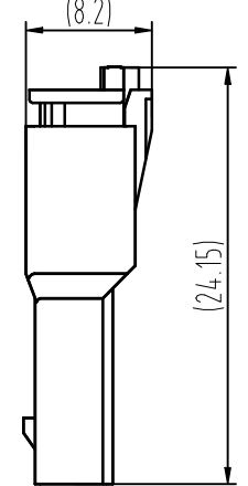
Assembly view (TJC2509-nAR&TJC2509B-nY) (DIM FYI)
