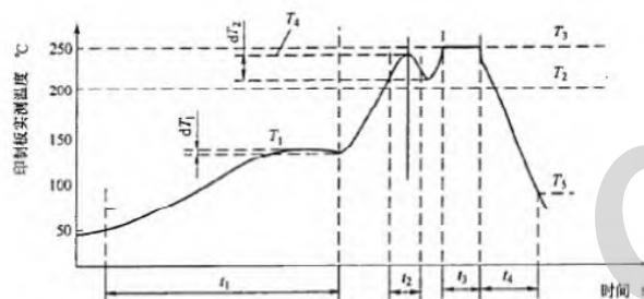
Pb-free Wave soldering Temperature profile
